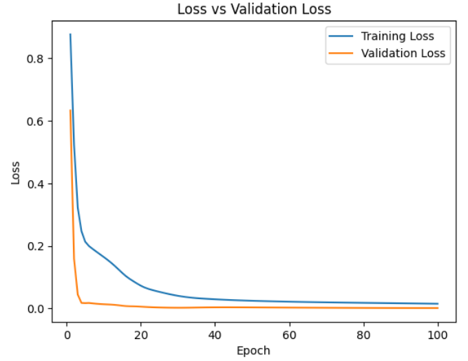
Fig. 2. Training and validation loss over 100 epochs for the LSTM model with seq_len = 10. Both curves converge without a large gap, suggesting limited overfitting.
